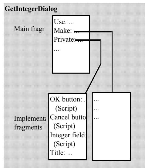
Figure 9: Structure of a dialog UIO
