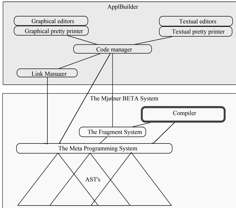
Figure 1: The architecture of the APPLBUILDER environment.
