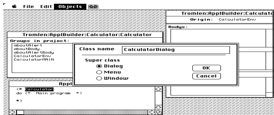
Figure 4: A new CalculatorDialog class inheriting from the general dialog class is added as the class description for the Calculator object.
